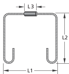
Typ/Type C/*CS
